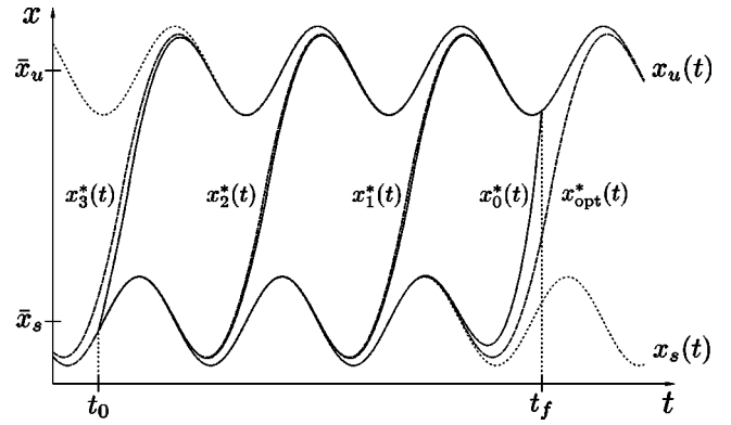
FIG. 3. Solid: The paths x_k^*(t) , k=0, \dots, K(t_f, t_0)=3 which minimize the action [Eqs. (36) and (37)] with boundary conditions (53). Dashed: The associated ‘‘master paths’’ x_{\text{opt}}^*(t + k\mathcal{T}) , implicitly defined via Eq. (54). Dotted: Stable and unstable periodic orbits x_s(t) and x_u(t) from Eq. (7). In this plot, t_f - t_0 has been chosen rather small. As t_f - t_0 increases, more and more intermediate paths x_k^*(t) appear which better and better agree with their associated master paths x_{\text{opt}}^*(t + k\mathcal{T}) . The depicted curves have been obtained for the additively driven piecewise parabolic potential [Eqs. (5) and (134)] with parameters A=0.5 , \Omega=1 , \lambda_s=-1 , \lambda_u=1 , \Delta V=1 , t_0=-12 , t_f=7.5 (dimensionless units).
